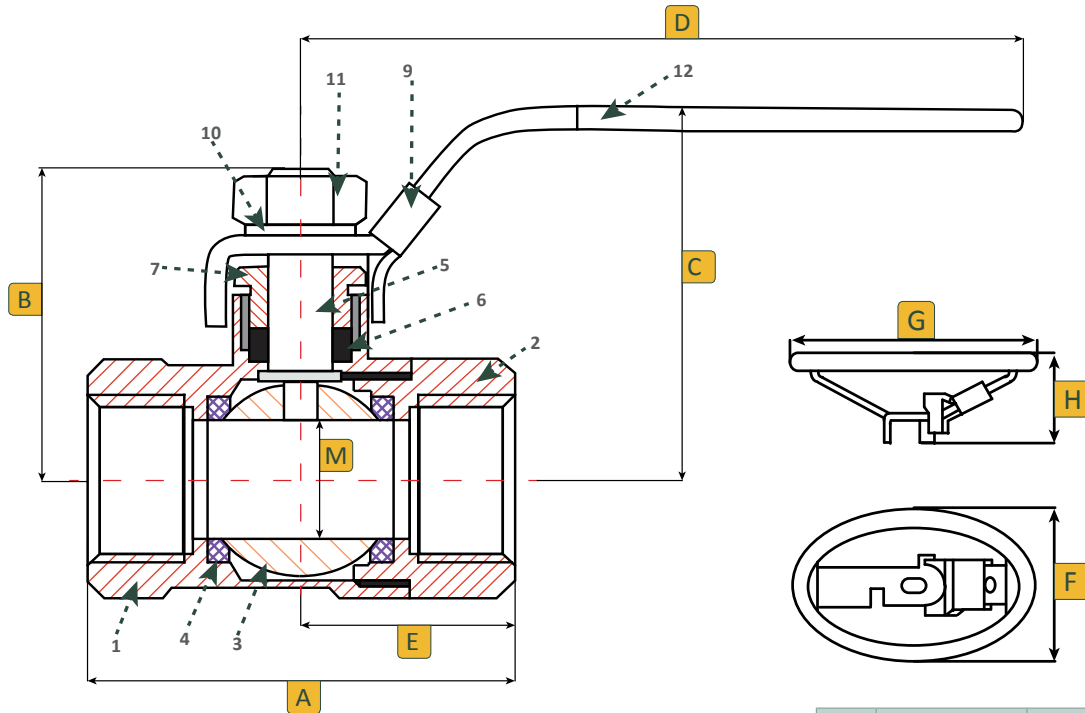
Dimensions (Inches)
