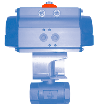
SB-CS with Quadrant C-Series Pneumatic Actuator
