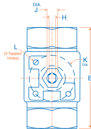
TOP VIEW (Handle Removed)
